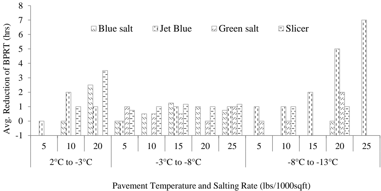
LOS Improvement Stratified by Temperature Rang (missing points indicate data not covered)
