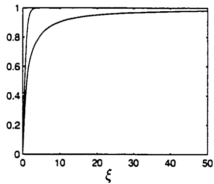
Figure D.1: The left hand side of Eq. (D.24) versus the right hand side. The upper curve is \tanh \xi whereas the lower curve is the sum.
