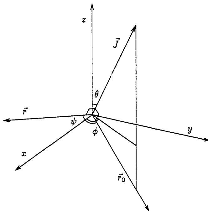
Figure 4.1: The angles involved in the location of the coherent state.
