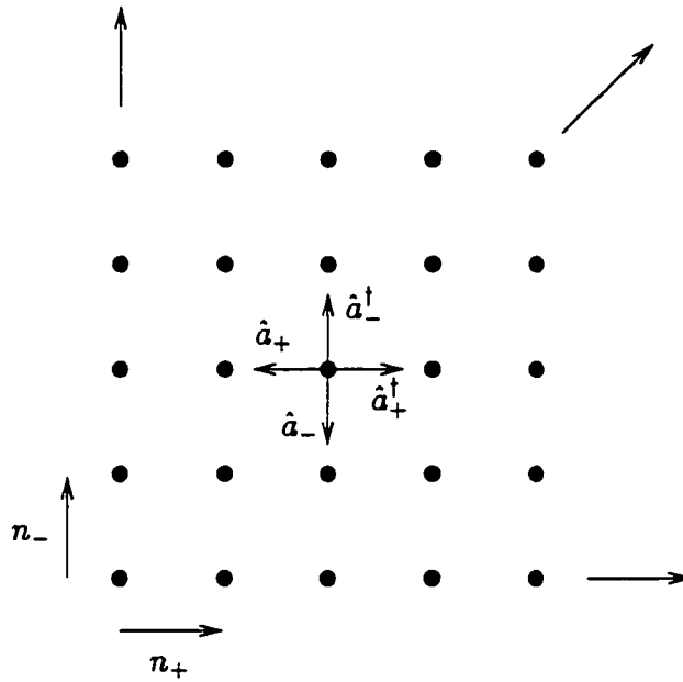
Figure B.1: Bosonic creation and annihilation operators.
