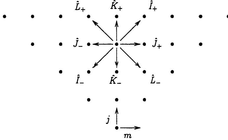
Figure B.2: Angular momentum ladder operators, acting on states |j, m\rangle with integer j .
