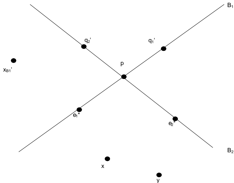
Figure C.1: Finding a length minimizing path
