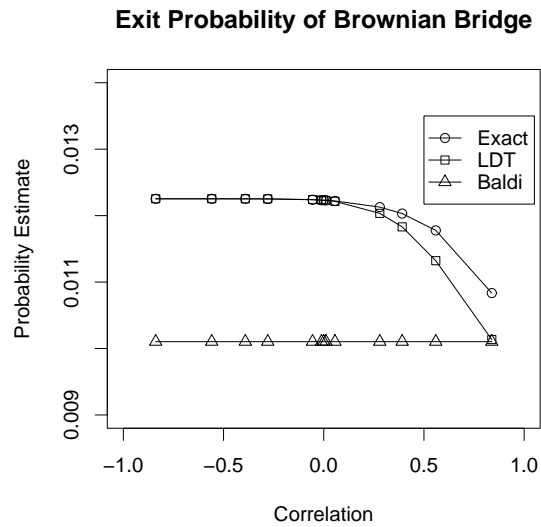
Figure 2.5: Estimates of Exit Probability for Case 4 with T = 0.5
