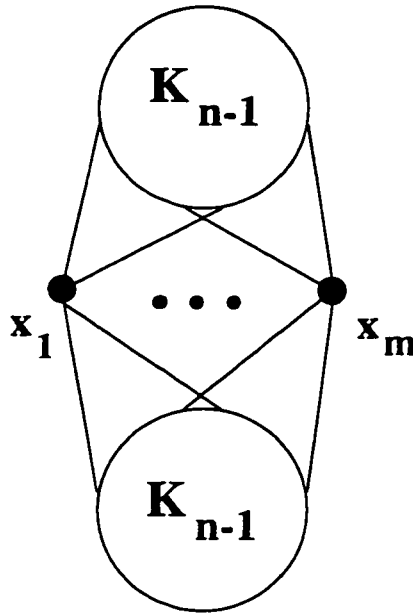
Figure 4.5: S_{m,m} .
