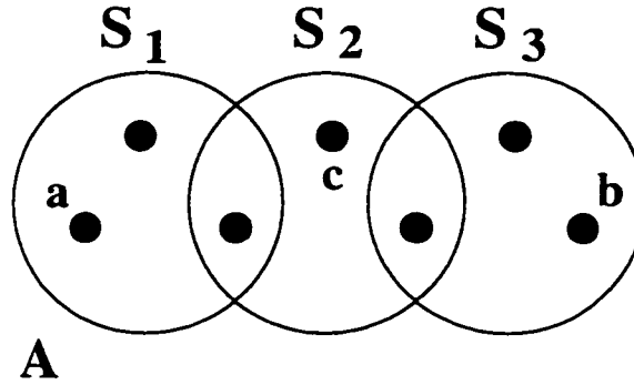
Figure 4.2: The 3-uniform hypergraph A .
