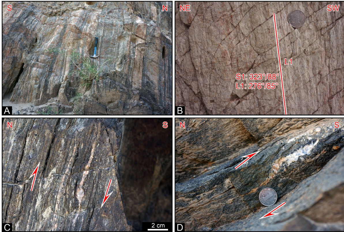
Figure 5. Field photos of D1 structures from domain A. All surfaces are subvertical. A: Striped gneiss with compositional layering (S1) defined by alternating light colored layers of granitic composition and dark layers that are biotite and amphibolite rich. B: Mica–quartz schist with a steeply plunging stretching lineation (L1) developed on the subvertical S1 foliation. C and D: \sigma -type structures indicating top-to-SE movement.
