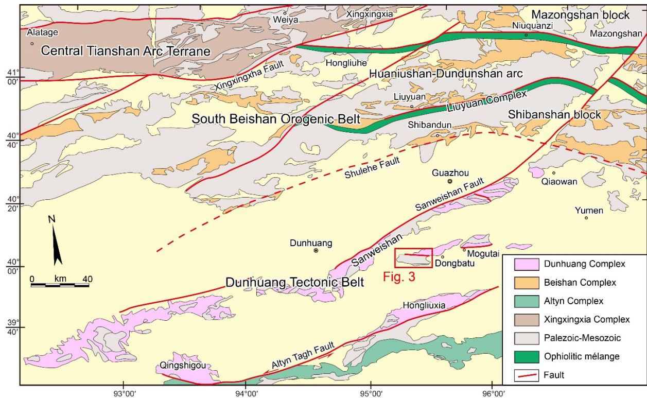
Figure 2. Simplified geological map of the Dunhuang Tectonic Belt and Beishan orogenic collage (modified after Xiao et al., 2010; He et al., 2014; Zhao et al., 2016; Wang et al., 2016). Area of this study (Fig. 3) is indicated.
