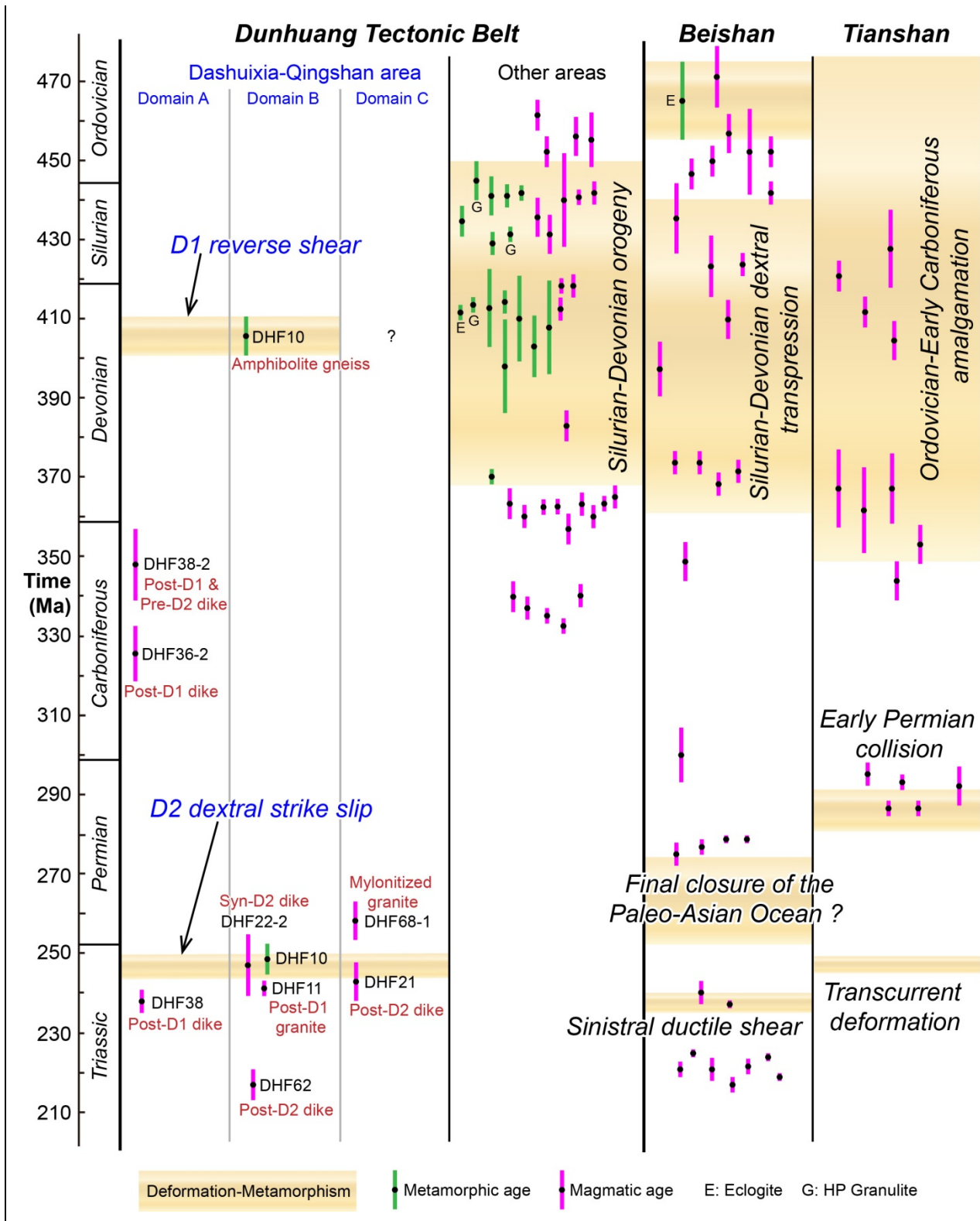
Figure 15. Diagram summarizing U–Pb age constraints on the timing of D1 and D2 deformation within the three domains in the study area. For comparison, data from other areas of the Dunhuang tectonic belt and the Beishan and Tianshan orogens are also indicated.
