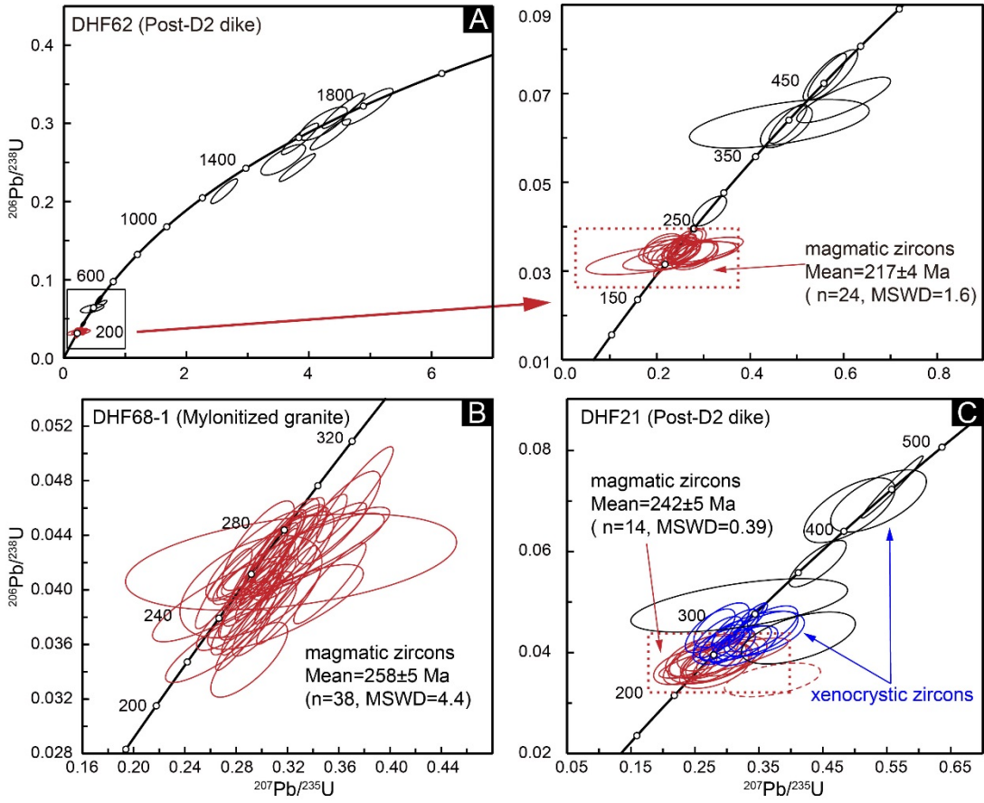
Figure 13. Zircon U–Pb concordia diagrams.
