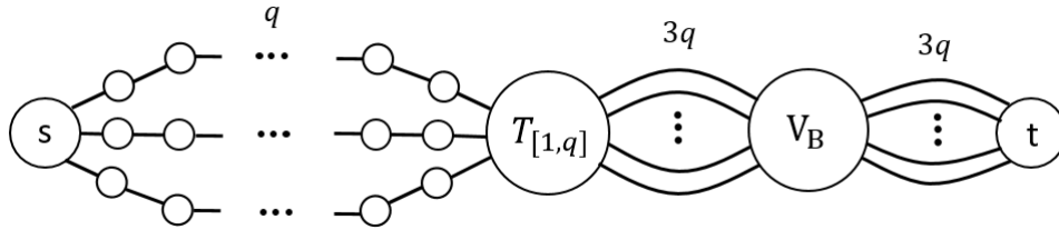
Figure 3: The subgraph H when the 3DM instance has q disjoint triplices.
