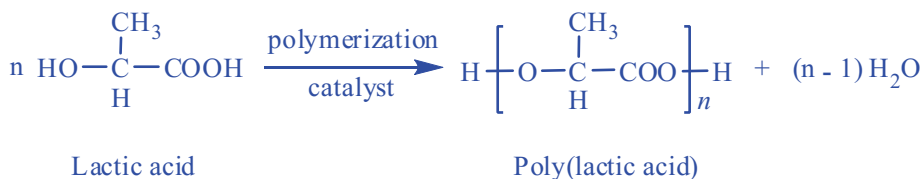
Scheme 2. Direct polymerization.
