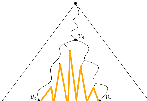
Figure 3.1: A range tree showing the path followed by a query for an interval [\ell, r] which splits at v_s , and the subtrees which fall within the query range between leaves v_\ell and v_r .
