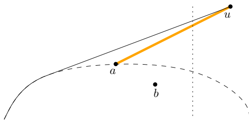
Figure 4.3: u kills a . The dotted line is the median vertical line and the dashed line was part of the convex hull before u was inserted. The point b must be below the bold line segment \overline{au} .
