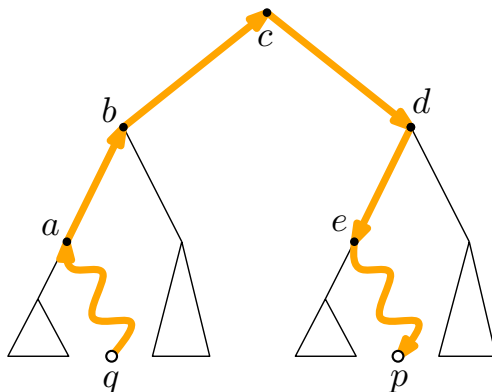
Figure 3.2: A search path finding the successor p of a point q is shown in bold . The search is divided into an “up” phase followed by a “down” phase.
