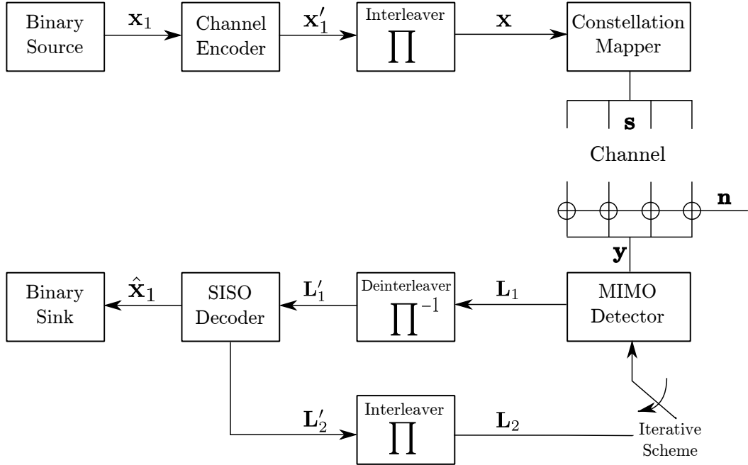
Figure 2.3: Transmitter and receiver in iterative detection/decoding for MIMO systems
