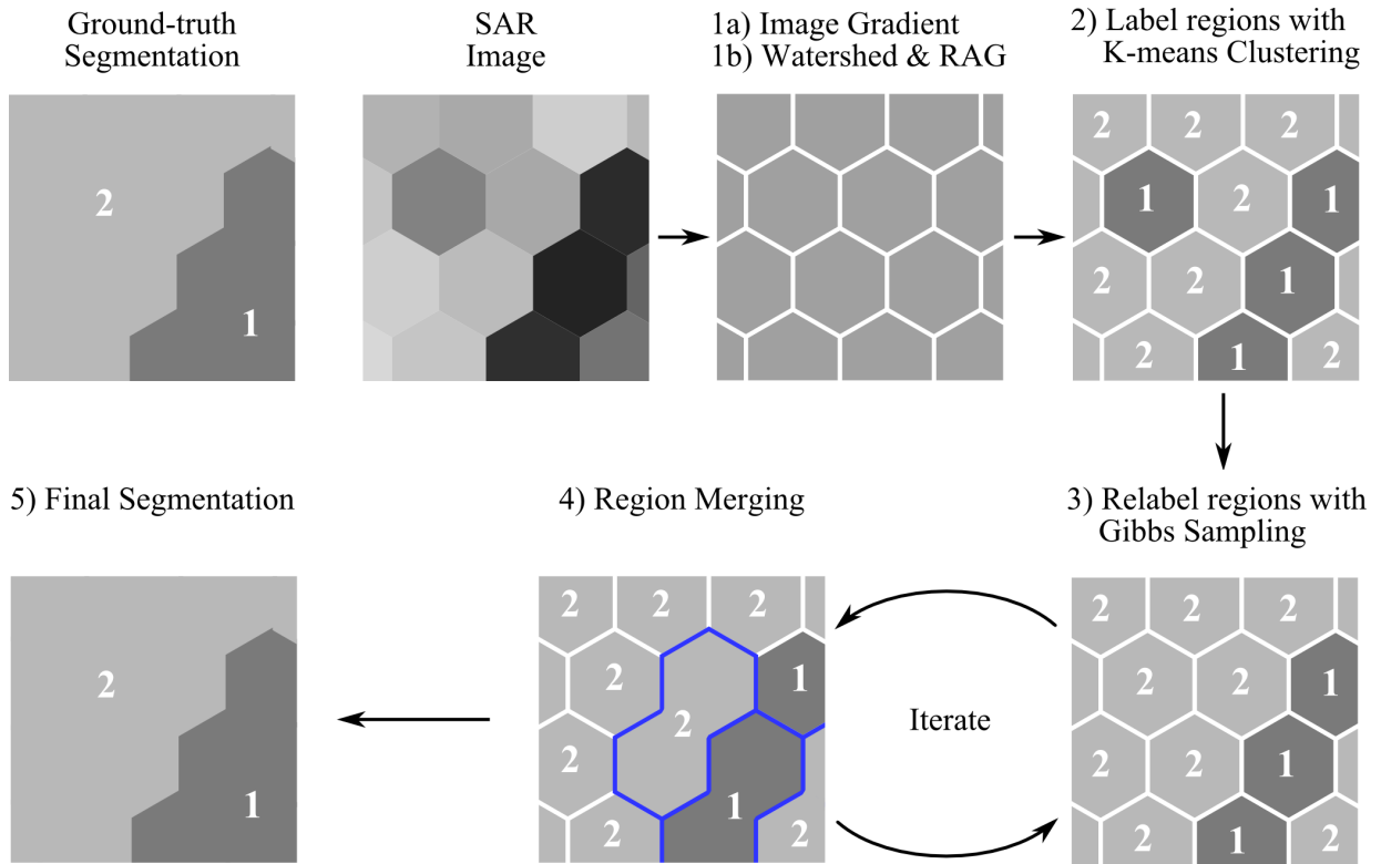
Figure 2.5: Major steps of the MIRGS algorithm. To initialize the system, MIRGS computes the 1a) image gradient, 1b) generates the watershed regions, the region adjacency graph (RAG) and 2) the initial segmentation with K-means. The 3) relabeling and 4) merging processes follow and are repeated for a user-specified number of iterations until the 5) final segmentation is produced.
