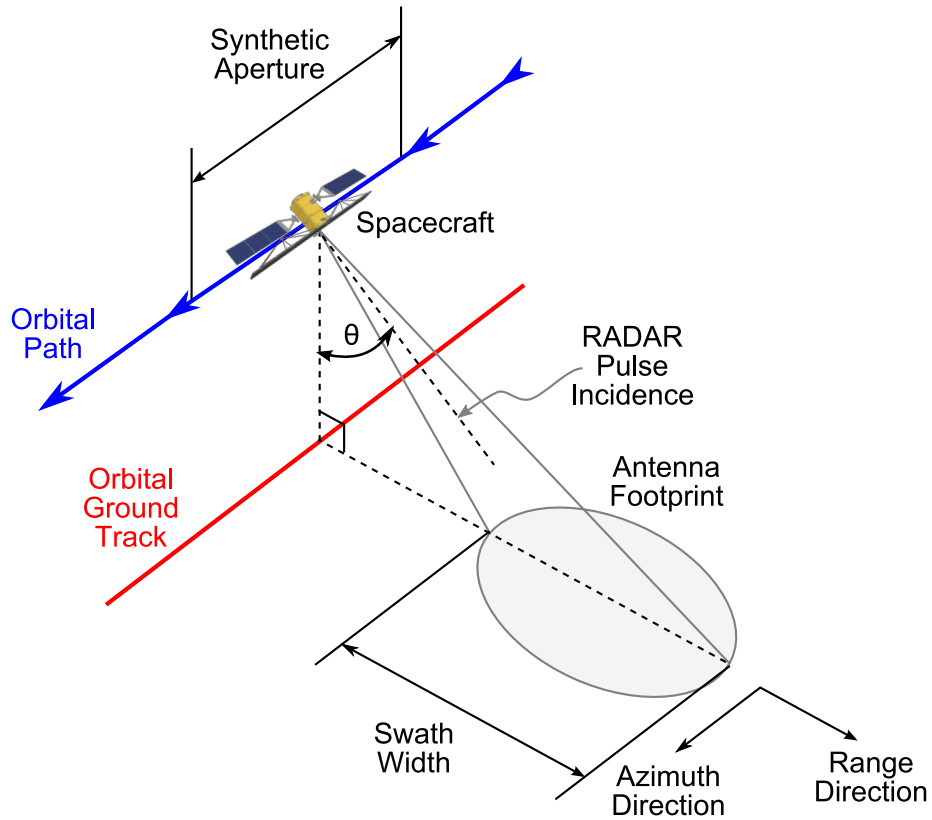
Figure 2.2: A diagram explaining the operation of SAR, adapted from [45]. The spacecraft sends a pulse of RADAR energy at the Earth's surface, which is reflected back and received as backscatter. The motion of the spacecraft creates a synthetic antenna aperture that is larger than the size of the antenna. The incidence angle \theta defines the angle to any ground range, which is the distance from the orbital ground track.
