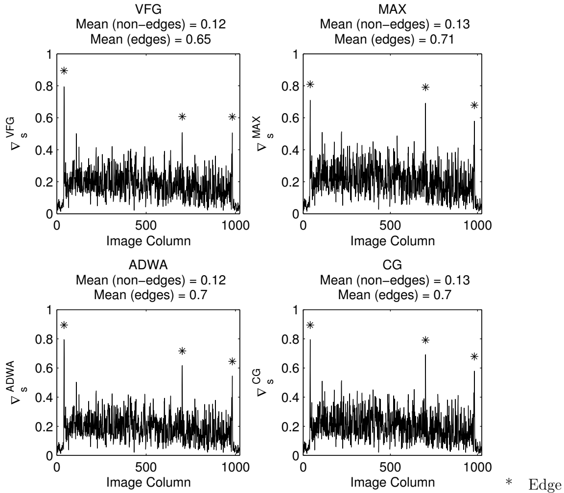
Figure 3.1: VFG, MAX, ADWA and CG gradient combination methods for a noisy synthetic two-channel image with step edges. Mean (non-edges) indicates the mean gradient value over all non-edge pixels with lower being better. Mean (edge) indicates the mean gradient value over all edges pixels, with higher being better.
