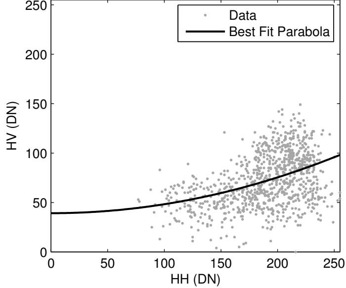
Figure 3.6: A least-squares fit of a parabola to the HH & HV data points in feature space. The data points shown here correspond to the real image (Figure B.1).
