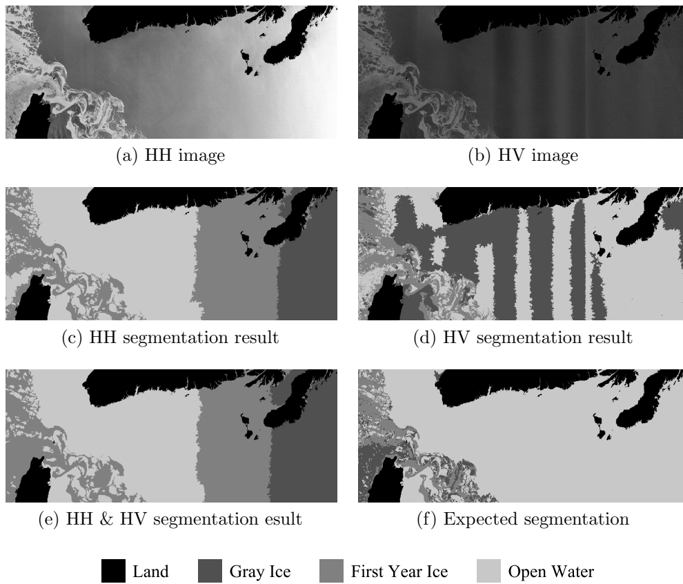
Figure 2.9: Segmentation results using MIRGS applied to a full scene R2 image. The incidence angle variation of open water causes both IRGS and MIRGS to produce incorrect segmentation results. The open water portion should not be split into multiple sections.
