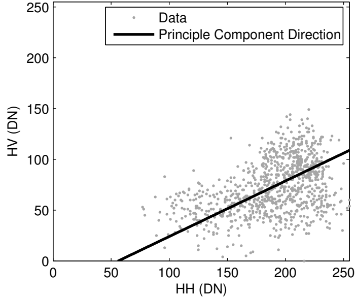
Figure 3.5: The line represents the principal component direction onto which the data points are projected during PCA. The data points shown here correspond to the real image (Figure B.1).
