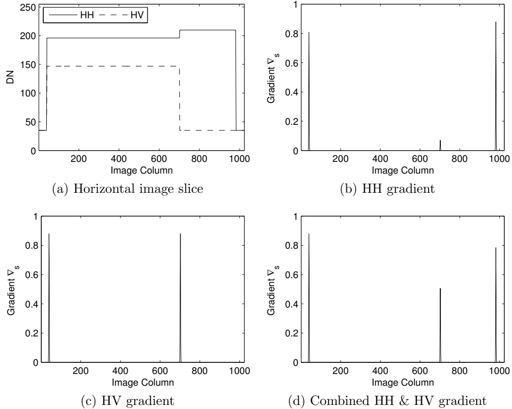
Figure 2.8: An example showing the dual-polarization performance of the joint VFG gradient method. (a) A plot of the intensity in digital numbers (DN) of a horizontal slice through a synthetic dual-polarization image with step edges shows that some edges are strong in HH and some are strong in HV. (b) Gradient through the same slice derived from the HH channel does not pick up the middle edge which is low contrast in HH. (c) Gradient from the HV channel does not pick up the right edge but assigns high relative strength to the left and middle edges. (d) The combined gradient picks up all edges, but the relative strength is strongest for the edge that is in both images even though all edges are expected to be equally meaningful.
