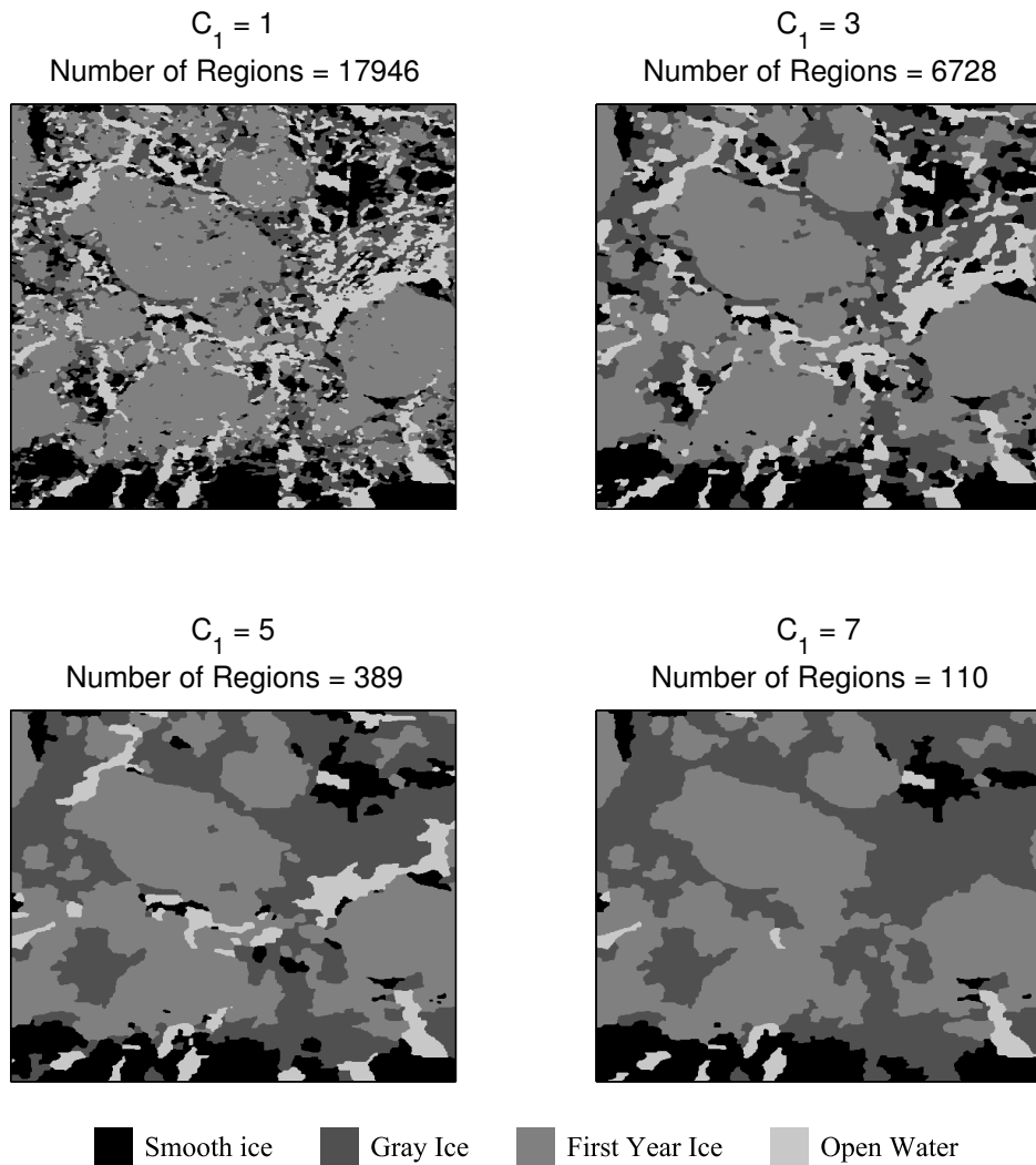
Figure 4.1: Segmentation results obtained for the real image (Figure B.1) using HH & HV with VFG gradient (the best feature set according to Table 4.2) at different values of C_1 . The effect of larger C_1 is to increase the amount of merging. C_2 was fixed at 0.4.
