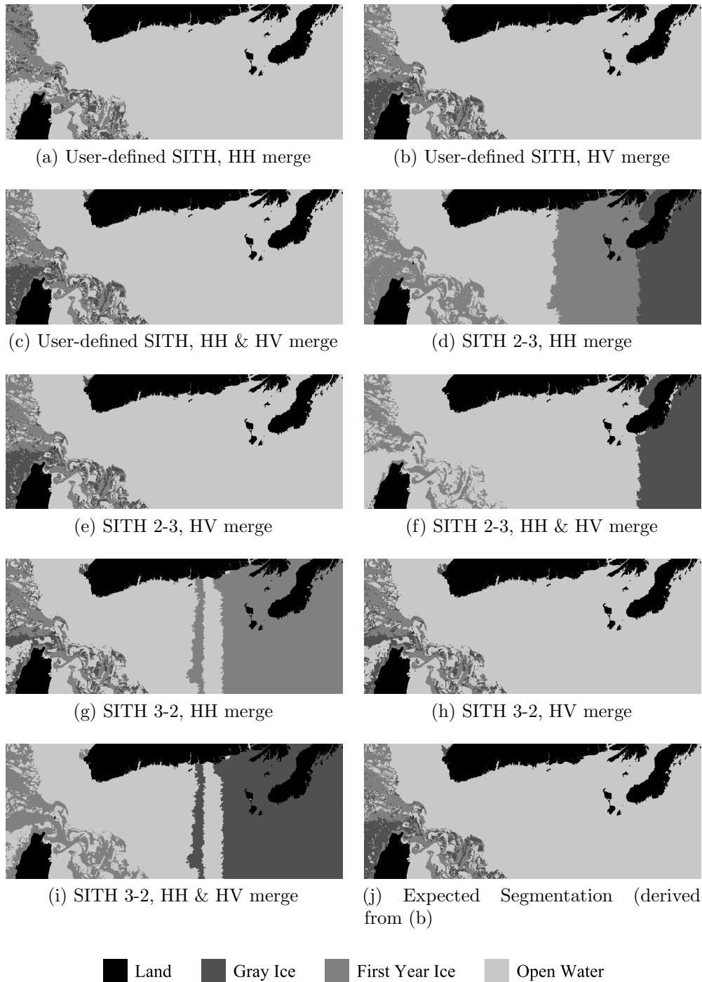
Figure 4.14: The incidence angle variation of open water can be handled by the selection of an appropriate sea ice typing hierarchy followed by merging of extra segments using the Fisher criterion in an appropriate feature set. In the full scene image (Figure B.3), the user-defined hierarchy followed by merging using (b) HV only or (c) HH & HV works well. SITH 2-3 with merging on (e) HV also works. (j) The expected answer for comparison is derived from the user-defined hierarchy result.
