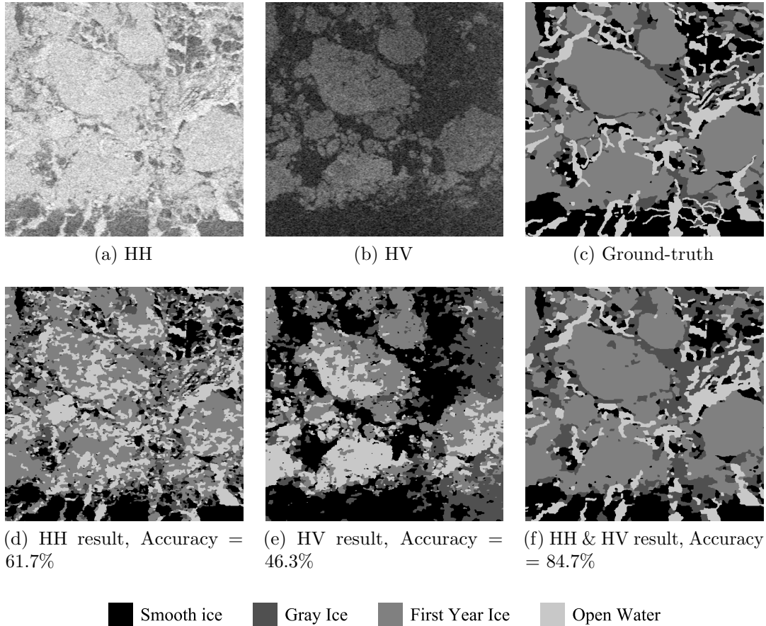
Figure 2.6: An evaluation of MIRGS with R2 data. A subimage from a R2 scene was selected for evaluating MIRGS using default parameters ( C1 = 3, C2 = 0.5 ) by comparison with a manually segmented ground-truth. The HH result shows ambiguities in the segmentation and the HV result is incorrect. Only the HH & HV result is accurate but it appears to lose details due to overmerging.
