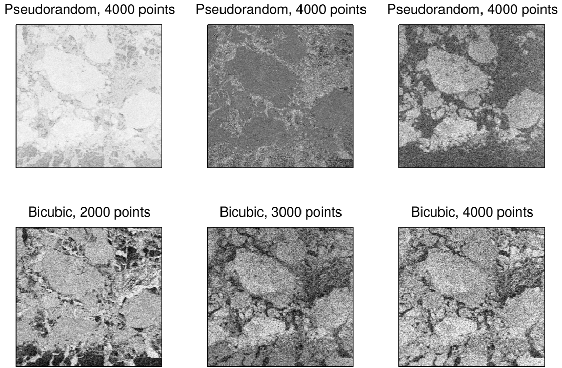
Figure 4.7: LTSA is not robust to picking different subsets of samples for use during the training phase since each sample subset produces a different fused image result.
