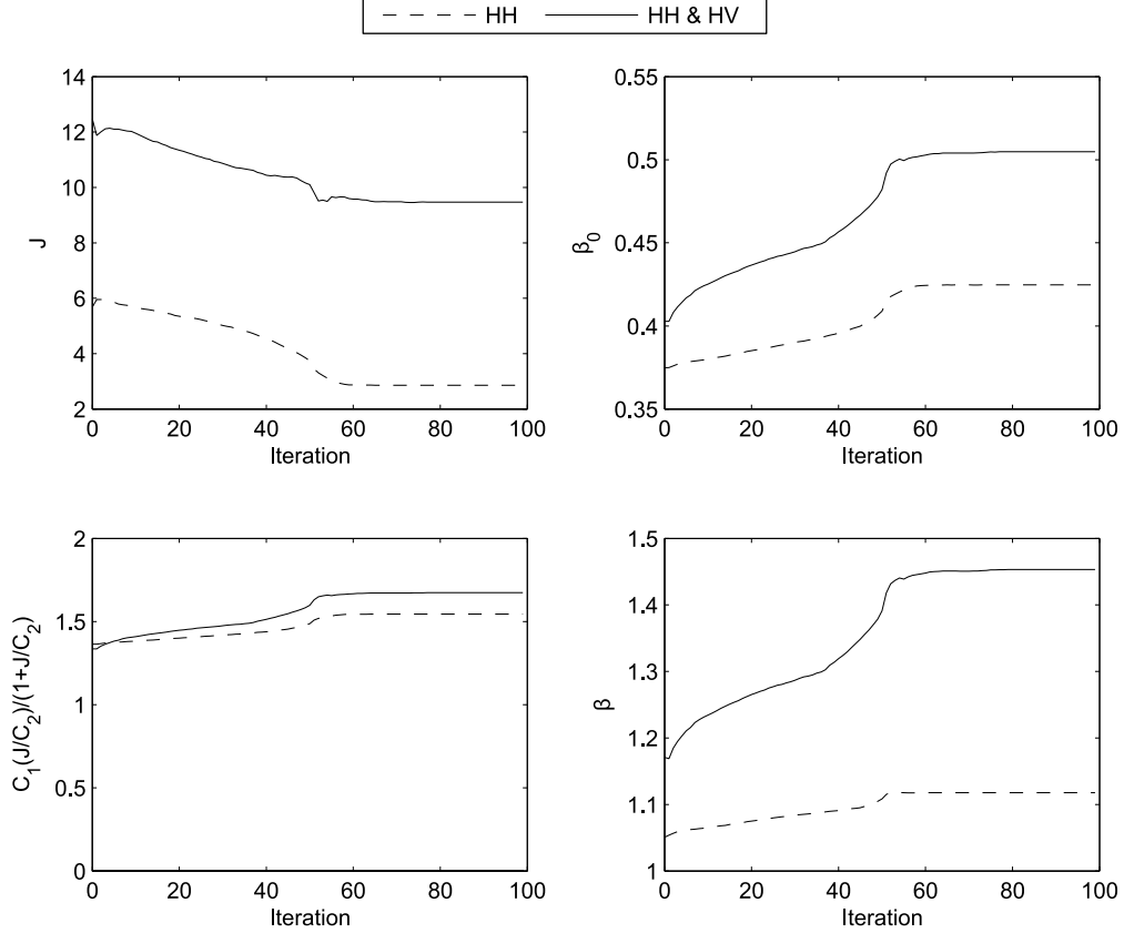
Figure 2.7: Comparison of the spatial context parameter \beta as a function of iteration between univariate and multivariate feature sets. The parameter \beta is affected by \beta_0 and the Fisher criterion J for the two least separable classes. The dual-pol data inherently causes more merging by causing larger \beta values for the same set of C_1 and C_2 . This is because the feature space separability is higher which causes larger J and \beta_0 values. These in turn cause \beta to be larger, in accordance with Equation 2.6.
