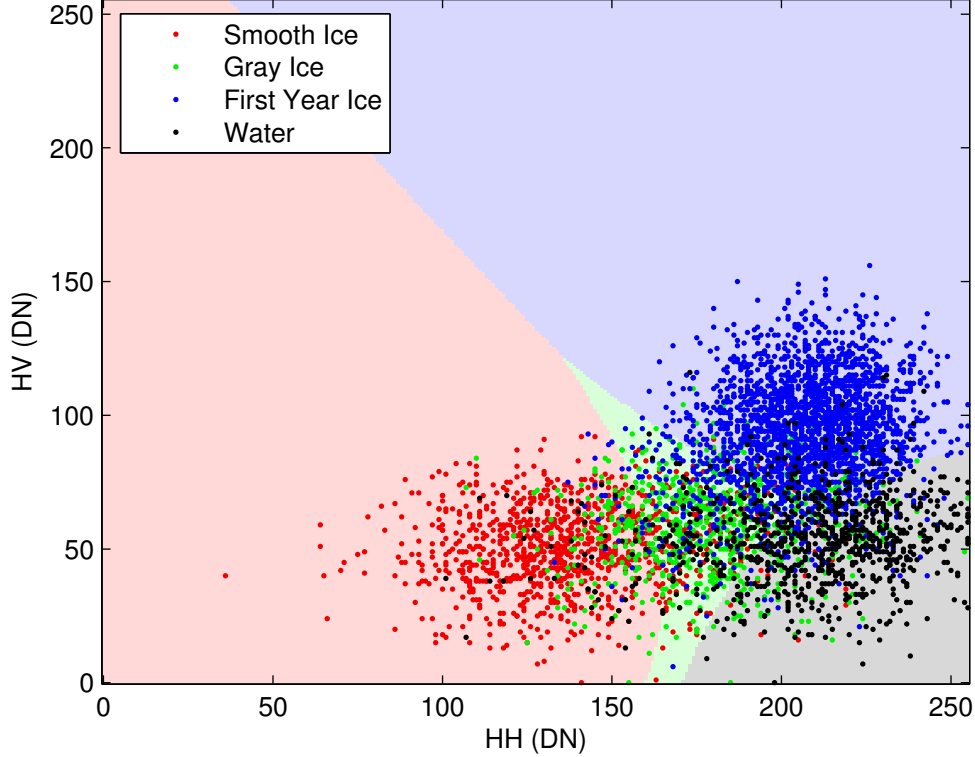
Figure 3.4: The HH & HV feature space plot of the real image (Figure B.1). Light shades in the background indicate the Gaussian maximum likelihood decision boundaries.
