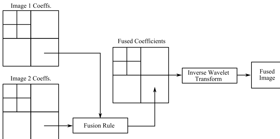
Figure 3.3: Wavelet image fusion is accomplished by decomposing the individual images using the wavelet transform, fusing the corresponding coefficient images into a single fused decomposition and then performing the inverse wavelet transform to obtain the fused image.
