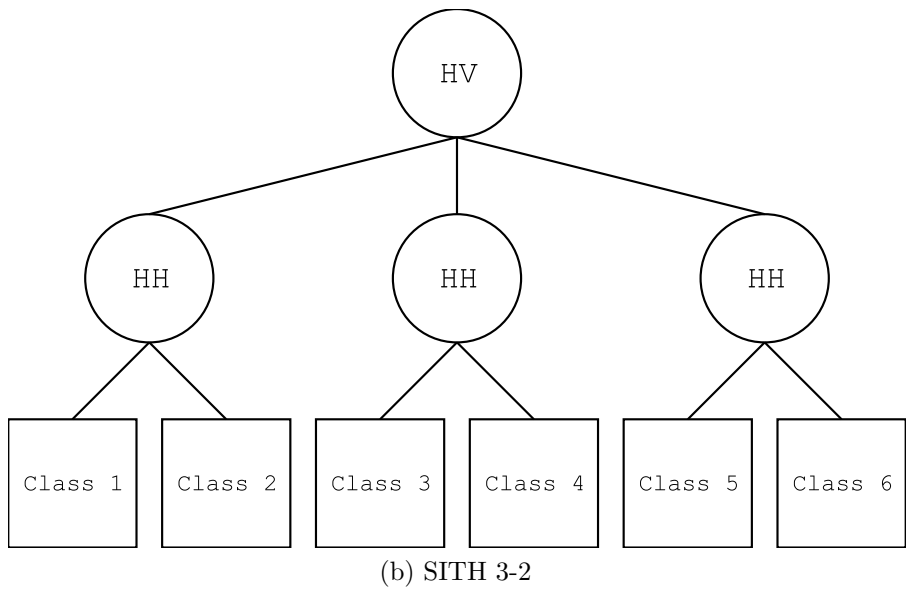
Figure 3.9: Two generic sea ice type hierarchies that were also tested.
