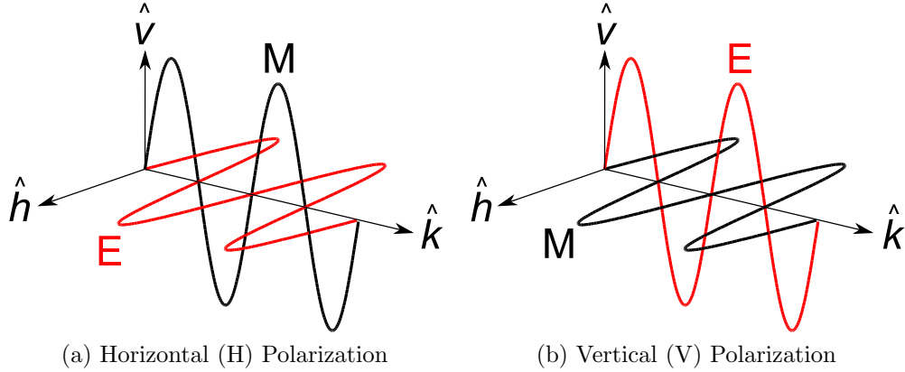
Figure 2.3: Waves of electromagnetic radiation consist of orthogonal electric (E) and magnetic fields (M) traveling in direction \hat{\mathbf{k}} . Linearly polarized waves, such as that used in SAR, have fixed directions for the fields. (a) Horizontally polarized waves have electric fields in the \hat{\mathbf{h}} direction. (b) Vertically polarized waves have electric fields in the \hat{\mathbf{v}} direction.
