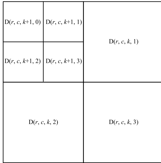
Figure 3.2: A two level wavelet multi-resolution decomposition. Level k contains three detail coefficient images D(r, c, k, 1 \dots 3) . Level k + 1 is the highest stage of this decomposition and contains an approximation coefficient image D(r, c, k + 1, 0) and three detail coefficient images D(r, c, k + 1, 1 \dots 3)
