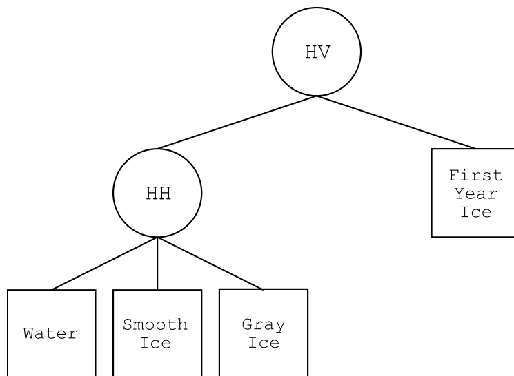
Figure 3.8: An example sea ice type hierarchy for hierarchical segmentation. The order of the branches from each channel from left to right indicates the brightness of each class in the channel from darkest to brightest.
