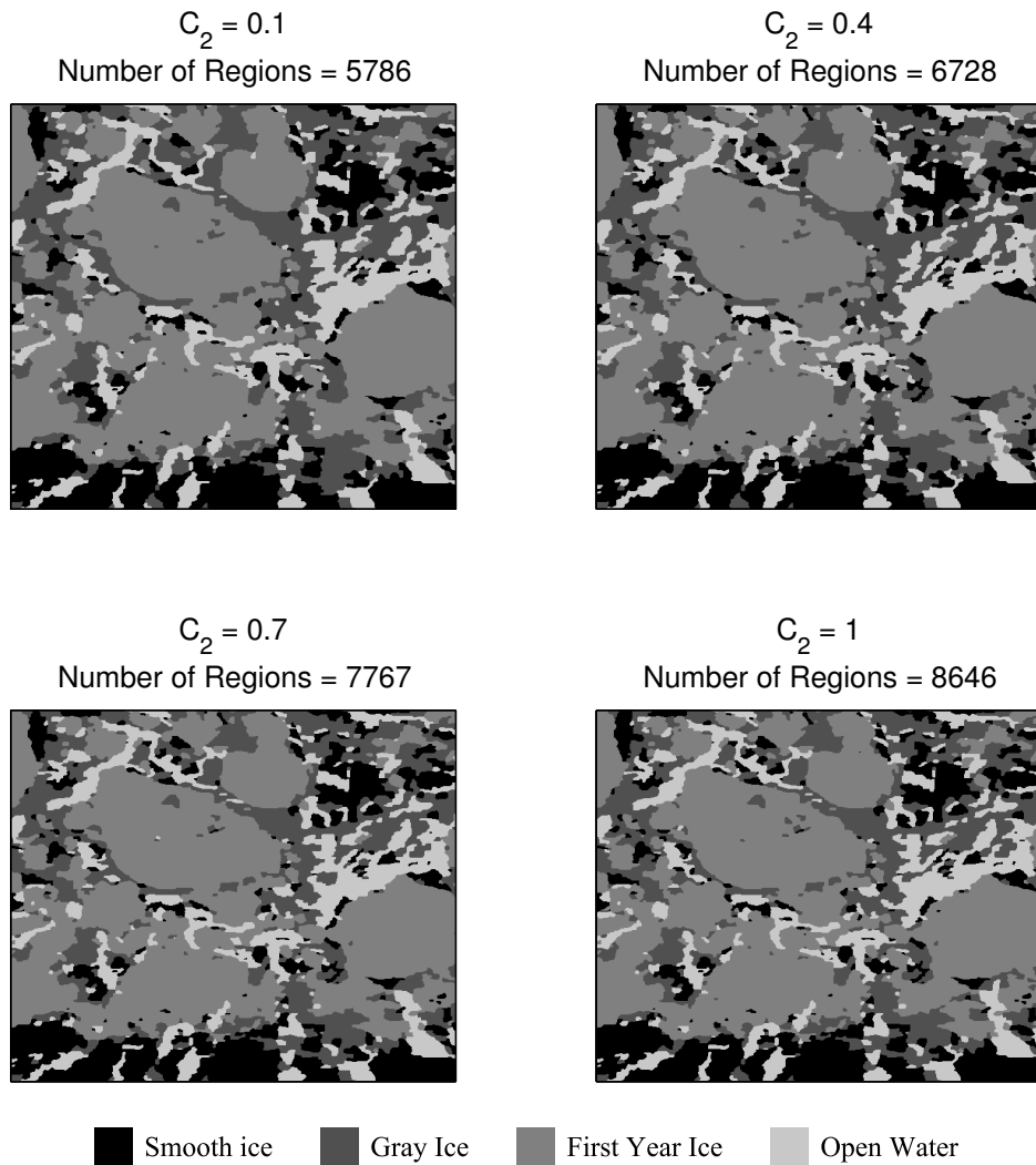
Figure 4.2: Segmentation results obtained for the real image using HH & HV with VFG gradient (the best feature set according to Table 4.3) at different values of C_2 . The effect of larger C_2 is to decrease the amount of merging. C_1 was fixed at 3.
