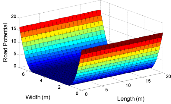
Fig. 5. Lane changing road potential field.
